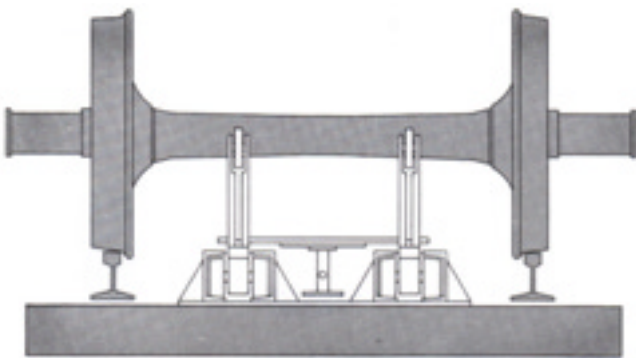
Double arm contacting axle. For draw bar pulls of 35,000 to 70,000 lbs.
