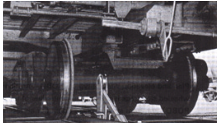
ROBOT arms ride in covered track between rails, rise to contact axle, side frame or coupler, according to design.
