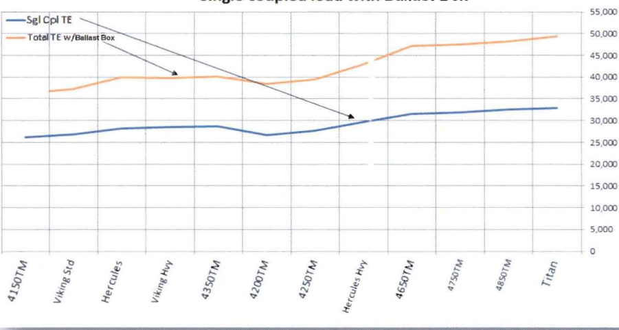
Tractive Effort Single coupled load with Ballast Box
