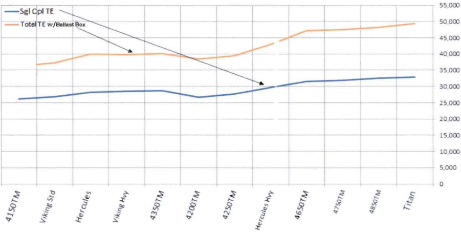
Tractive Effort Single coupled load with Ballast Box
